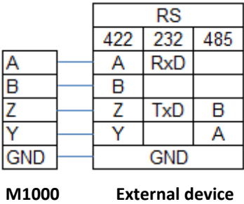
Wiring diagram for RS232, RS422; RS485
