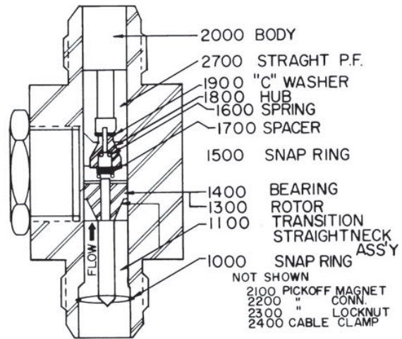
Figure 10: Models CLFC6...CLFF6
