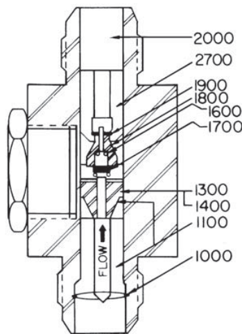
Figure 9: Model CLFB6
