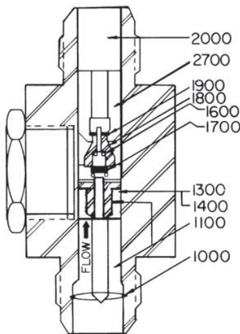
Figure 8: Model CLFA6
