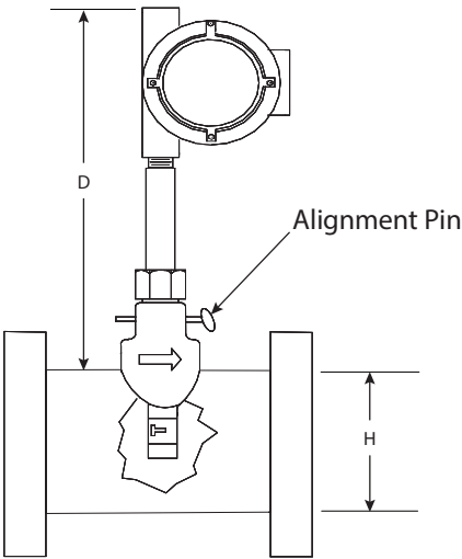
Figure 2: Compact meter inserted into pipe
