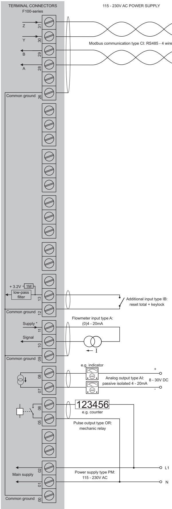
Configuration example F110-A-AI-CI-IB-OR-PM-XX-ZX
