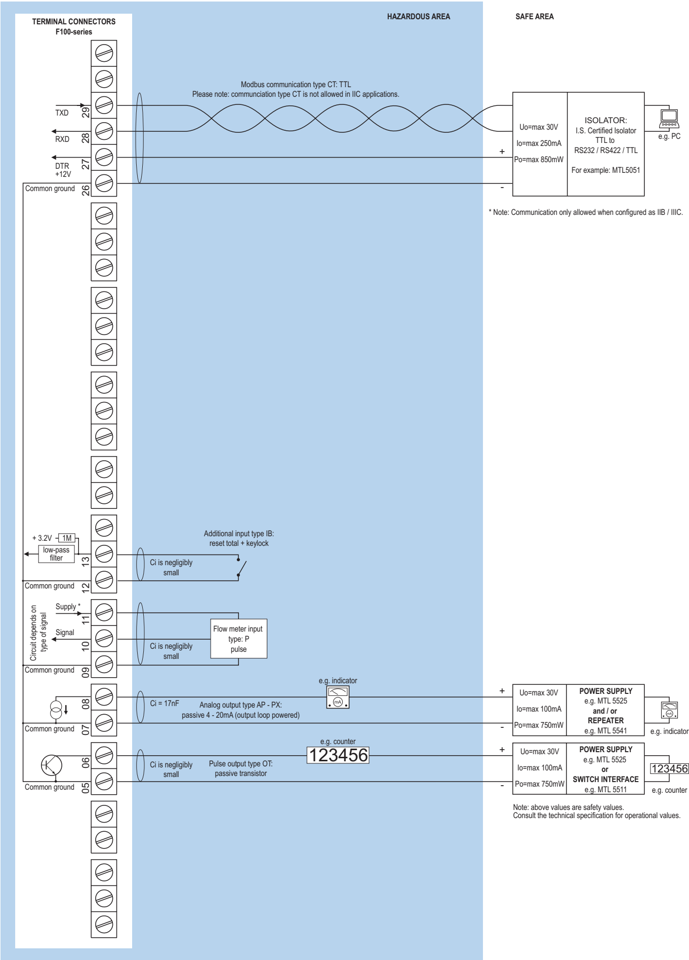
Configuration example IIB /IIIC and IIC - F110-P-AP-(CT)-IB-OT-(PX)-XI - Output loop powered
