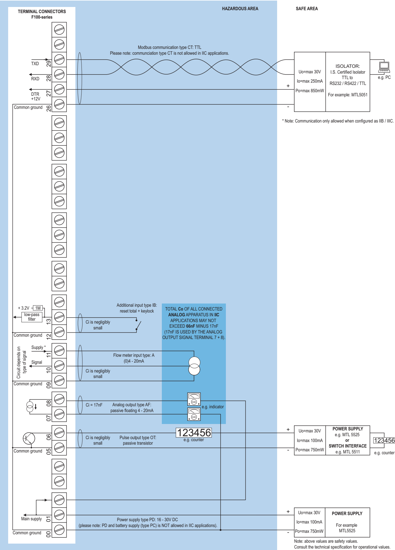
Configuration example IIB / IIIC and IIC - F110-A-AF-(CT)-IB-OT-PD-XI - Power requirement 16 - 30V DC
