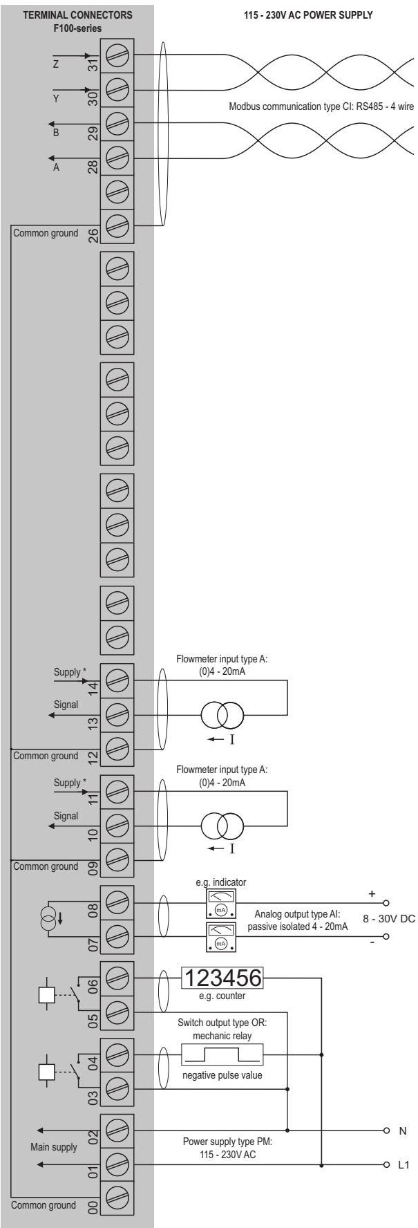
Configuration example F116-A-AI-CI-OR-PM-XX-ZX
