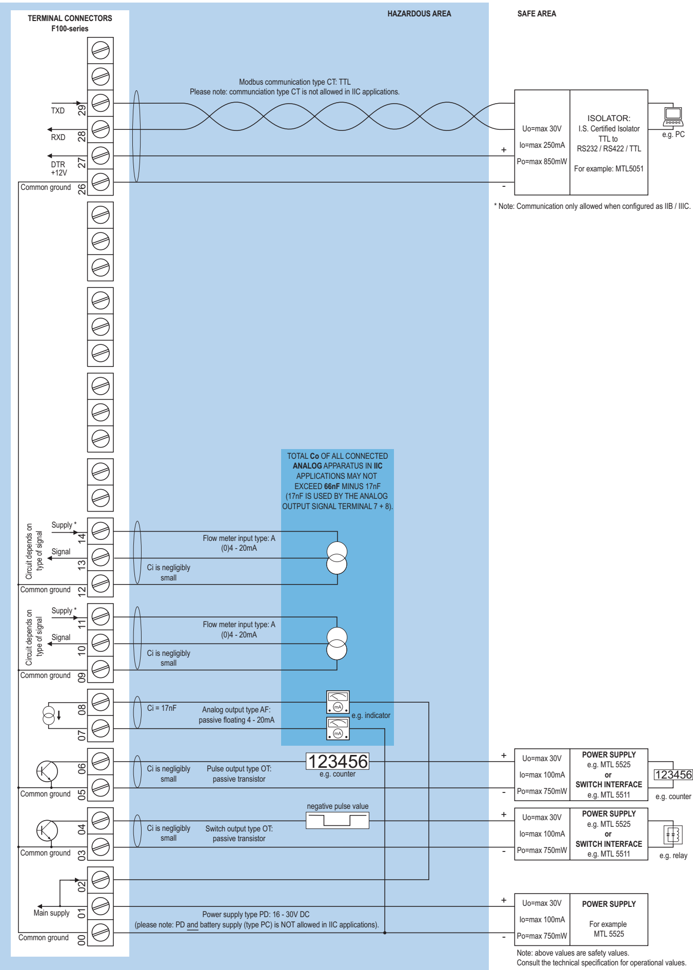
Configuration example IIB / IIIC and IIC - F116-A-AF-(CT)-OT-PD-XI - Power supply 16 - 30V DC
