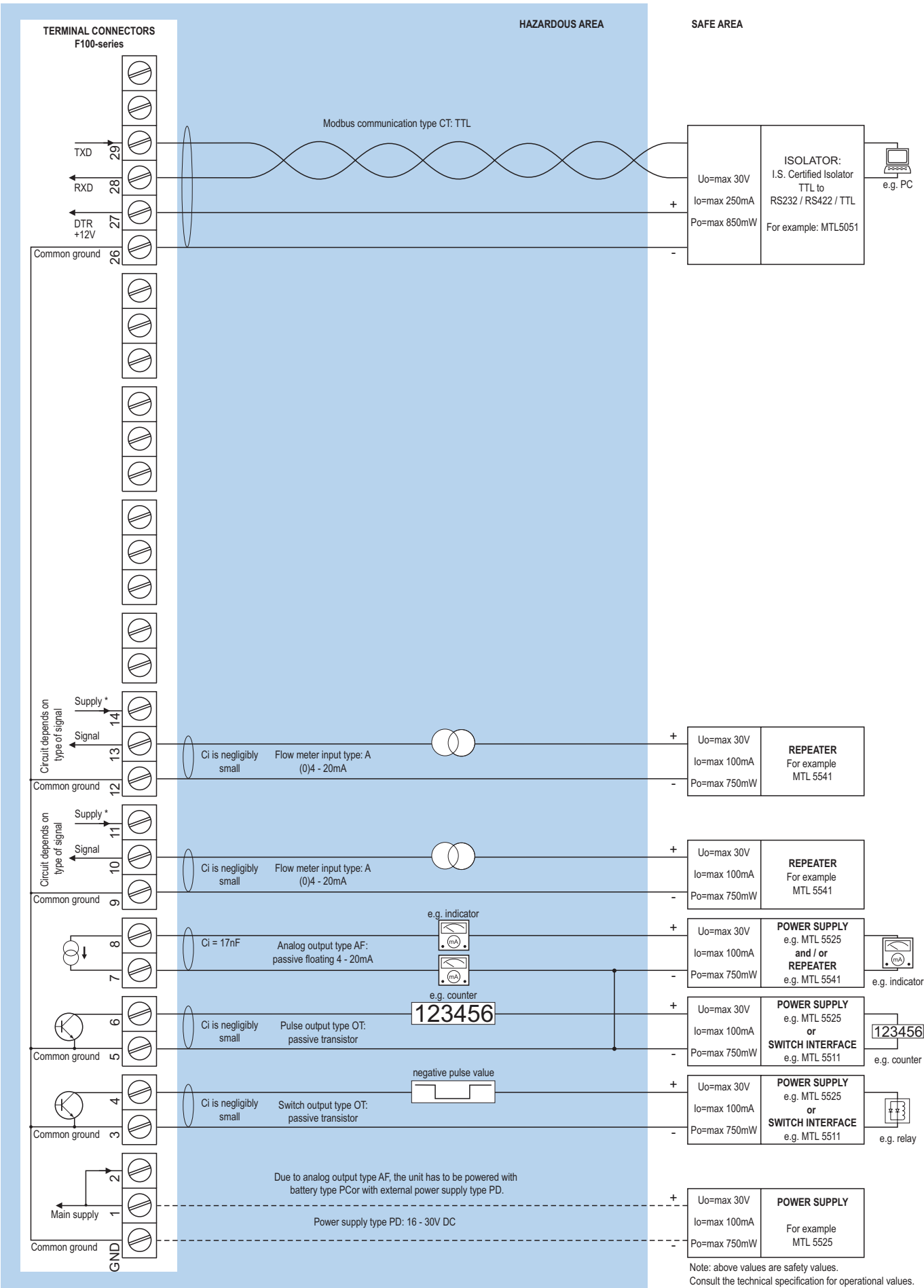
Configuration example IIB / IIIC - F116-A-AF-CT-OT-(PC)-(PD)-XI - Power supply 16 - 30V DC or battery powered
