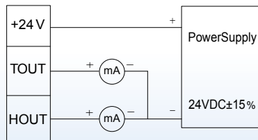
4-20mA (2-wire)
