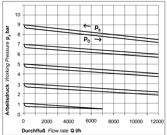
DN 10
